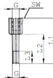
Stacking Bolt
